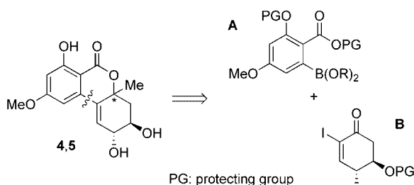
Scheme 1. Retrosynthetic analysis for altenuene and isoaltenuene.
