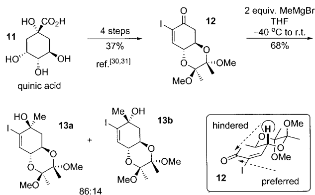
Scheme 4. Synthesis of the eastern building blocks 13a and 13b .
