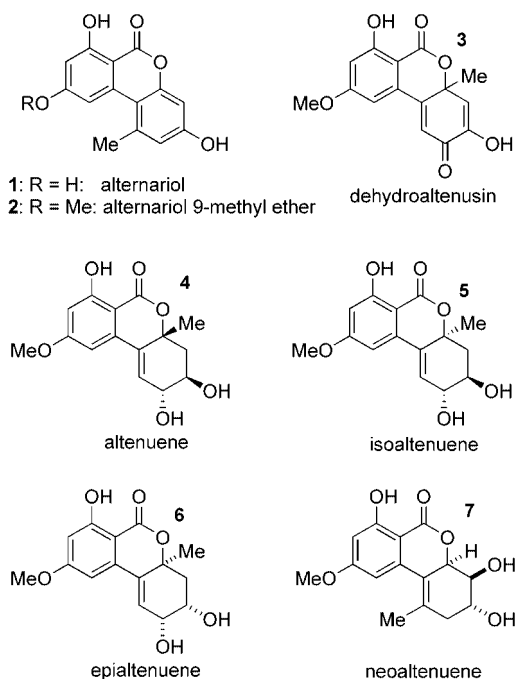
Figure 1. Toxins produced in alternaria fungi (absolute configurations for compounds 6 and 7 have not been reported; compound 3 racemizes under physiological conditions).
