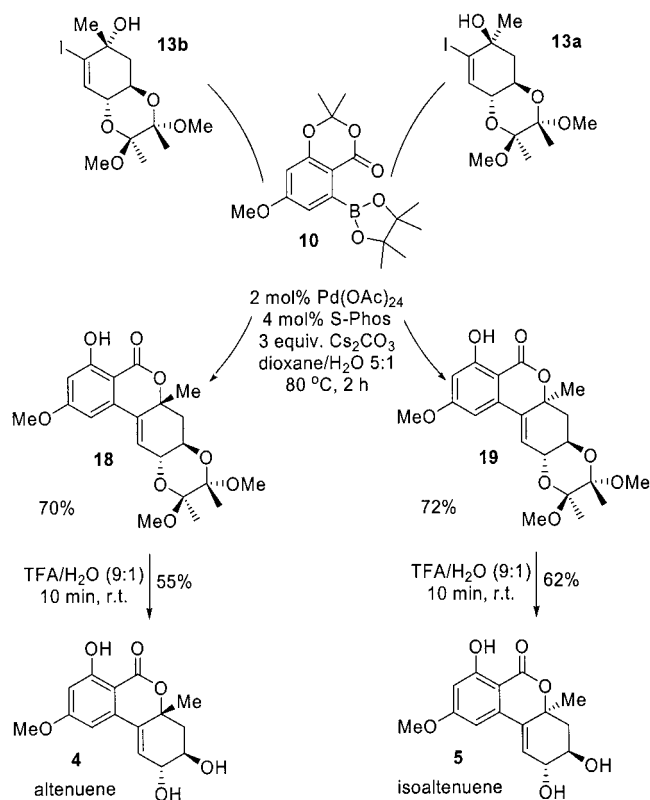
Scheme 5. Suzuki coupling of iodo alcohols and liberation of the natural products.
