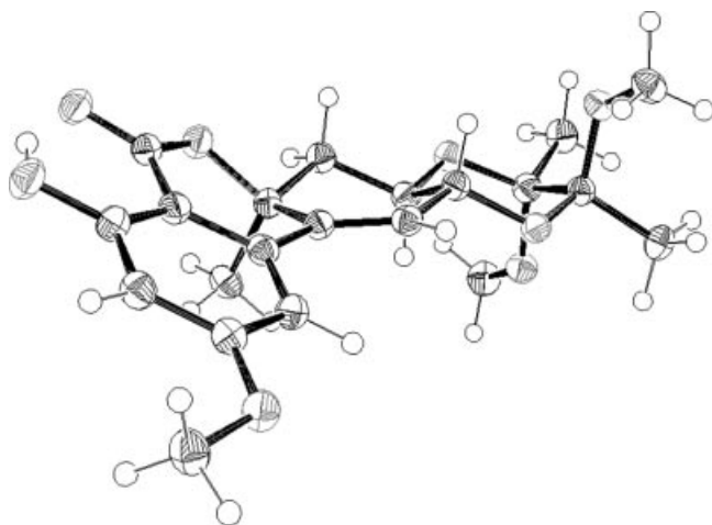
Figure 2. X-ray crystal structure of isoaltenuene derivative 19 . [35]
