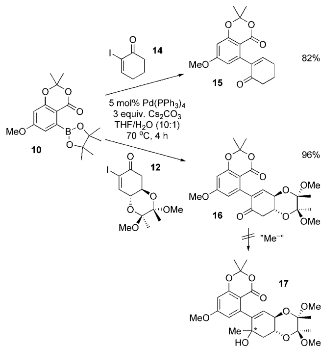
Scheme 3. Suzuki coupling of iodicyclohexenones.
