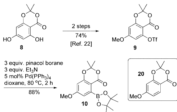
Scheme 2. Synthesis of the western building block 10 .
